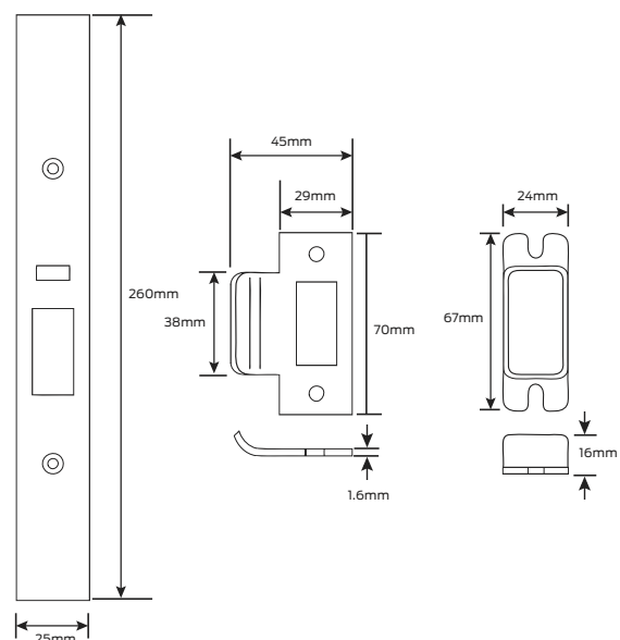
Forend & strike for wooden doors
